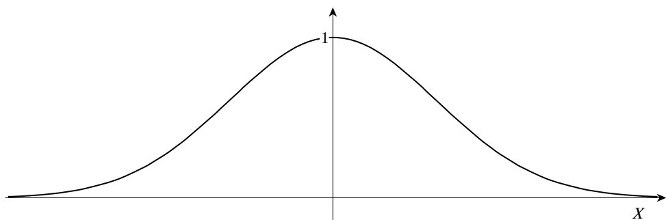
Figure 23.1: Graph of a basic Gaussian, e^{-\gamma x^2} for some \gamma > 0 .
