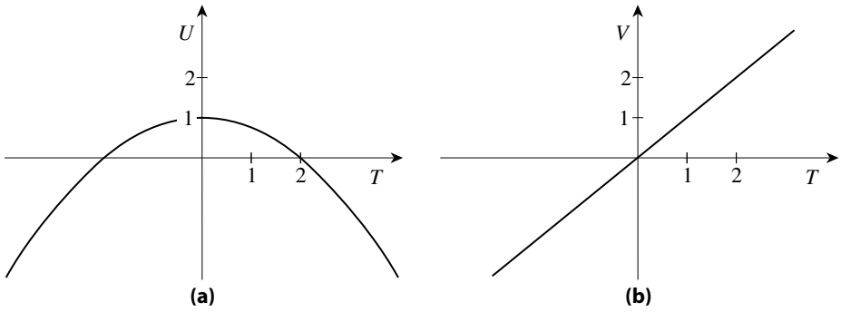
Figure 6.2: Graphing f(t) = \frac{1}{4}(2 + it)^2 : (a) the real part, u(t) = 1 - \frac{1}{4}t^2 , and (b) the imaginary part, v(t) = t .
