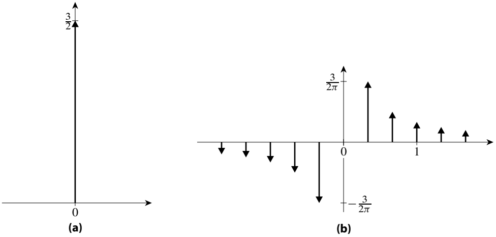
Figure 36.3: The (a) real part and (b) imaginary part of \mathcal{F}[\text{saw}_3] .
