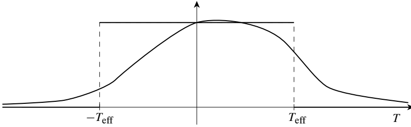
Figure 20.1: A function f and its effective duration for problem 20.19.
