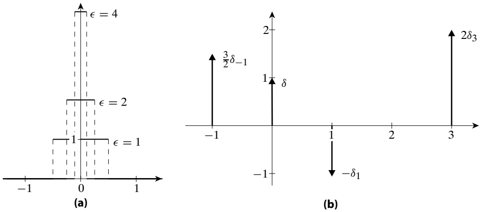
Figure 27.1: Delta functions — (a) viewed as a limit of pulse functions, and (b) graphically represented using vertical arrows.
