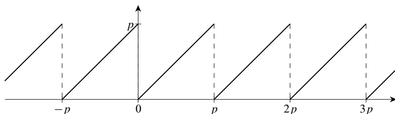
Figure 5.2: The graph of \text{saw}_p .
