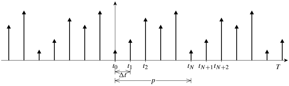
Figure 38.1: A periodic, regular array with spacing \Delta t , period p , and index period N . In this figure t_k = k\Delta t for k = 0, 1, 2, \dots
