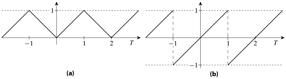
Figure 12.1: Two and one half periods of (a) \text{evensaw}(t) , the even sawtooth function for exercise 12.3 c, and (b) \text{oddsaw}(t) , the odd sawtooth function for exercise 12.3 d.
