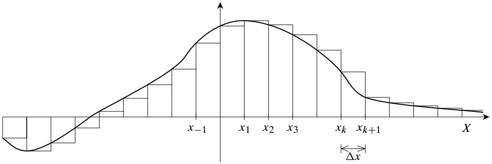
Figure 17.1: The graph of a real-valued function g and the rectangles for a Riemann sum approximation of \int_{-\infty}^{\infty} g(x) dx .
