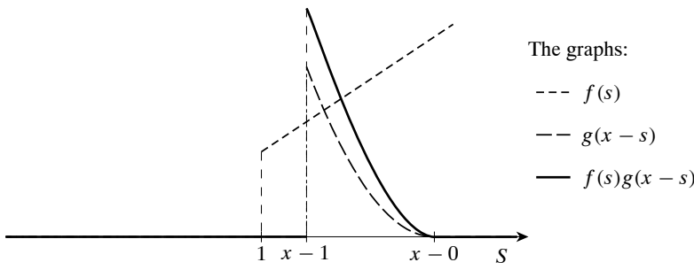
Figure 24.5: Step 6 in computing f * g(x) — superimposing g(x-s) on f(s) to help obtain y = f(s)g(x-s) when all singularities of g(s) are to the right of all singularities of f(s) .
