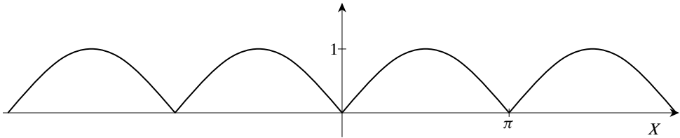
Figure 18.2: Graph of |\sin(x)| .
