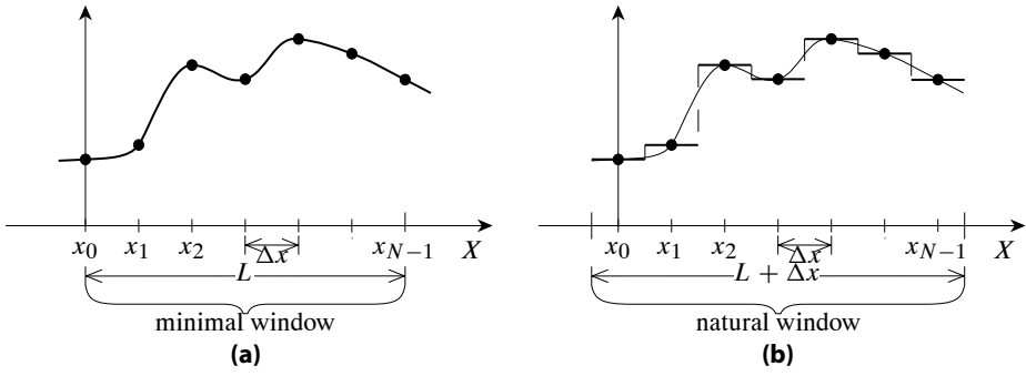
Figure 39.1: (a) The graph of an N^{\text{th}} order regular sampling with spacing \Delta x of a continuous, real-valued function f , with each dot representing a point (x_k, f_k) . (b) A simple piecewise continuous approximation to the function on the natural window on the sampling. In these figures x_k = k\Delta x .
