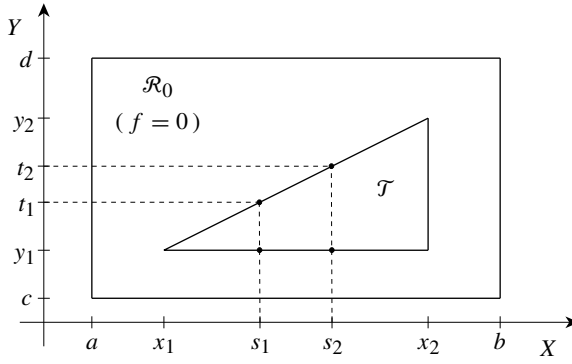
Figure 7.2: Figure for lemma 7.12.
