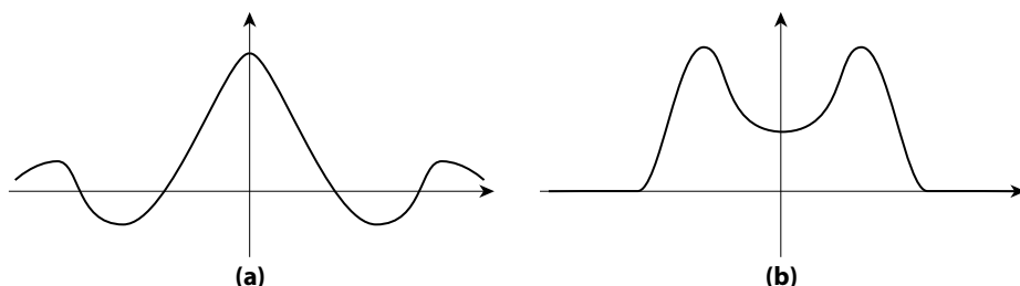
Figure 21.2: Graphs for exercise 21.17 with (a) being the graph of f and (b) being the graph of F .
