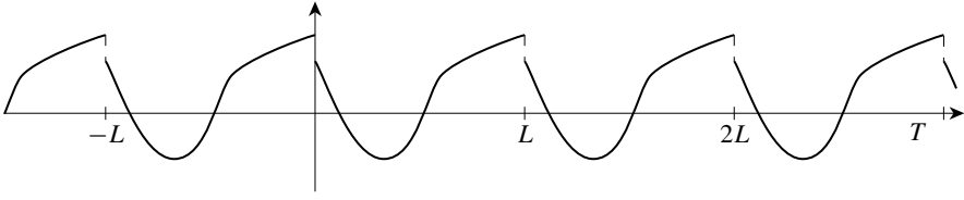
Figure 10.2: The basic periodic extension \widehat{f}(t) of the function graphed in figure 10.1.
