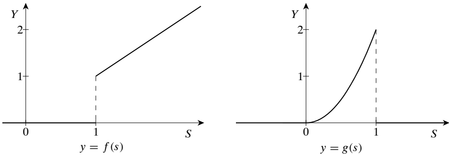
Figure 24.1: Step 1 in computing f * g(x) — graphing f(s) and g(s) separately.
