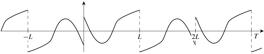
Figure 10.4: The odd periodic extension \widehat{f}_o(t) of the function graphed in Figure 0.1 (See also Figure 0.3).
