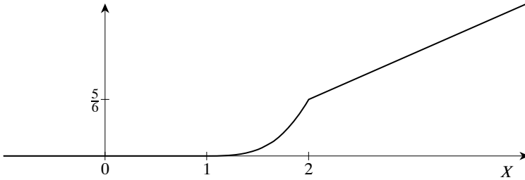
Figure 24.6: Graphing f * g(x) .
