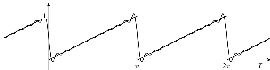
Figure 14.2: Graph of h superimposed on a partial sum for its Fourier series.
