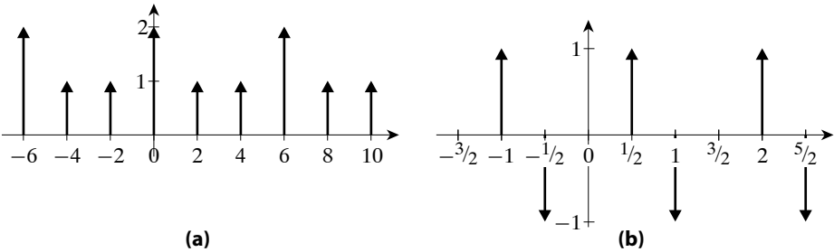
Figure 38.4: Two arrays of delta functions. (Two or more periods of each are sketched, and the coefficients are all integer valued.)
