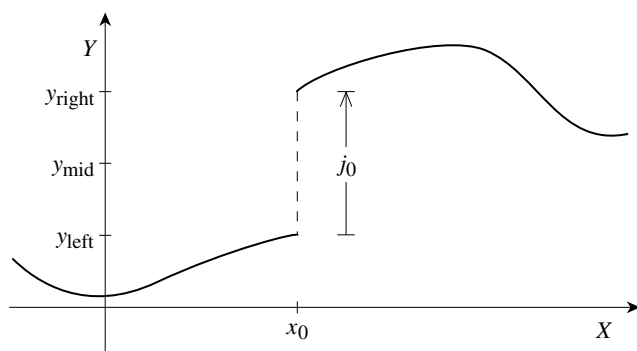
Figure 3.2: Generic jump discontinuity in f at x_0 with y_{\text{left}} = \lim_{x \rightarrow x_0^-} f(x) , y_{\text{right}} = \lim_{x \rightarrow x_0^+} f(x) and y_{\text{mid}} = “midpoint of the jump”.
