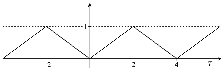
Figure 13.5: Two and one half periods of the even saw function for exercise 13.6 c.
