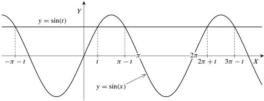
Figure 14.3: Values of x where \sin(t) = \sin(x) for a given t in (0, \pi/2) .
