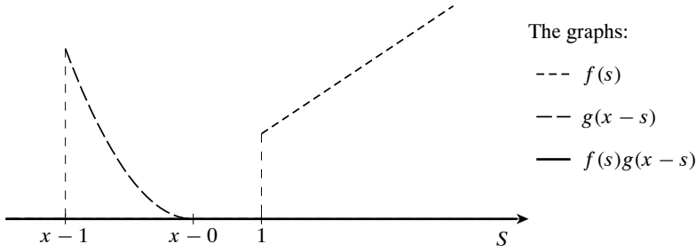
Figure 24.3: Step 4 in computing f * g(x) — superimposing g(x-s) on f(s) to help obtain f(s)g(x-s) when all singularities of g(x-s) are to the left of all singularities of f(s) .
