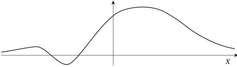
Figure 19.2: The graph of the function f(x) for exercise 19.18.
