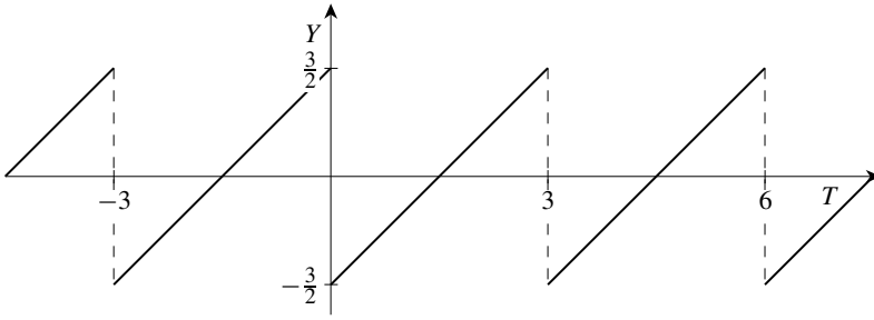
Figure 9.2: The saw function for example 9.5.
