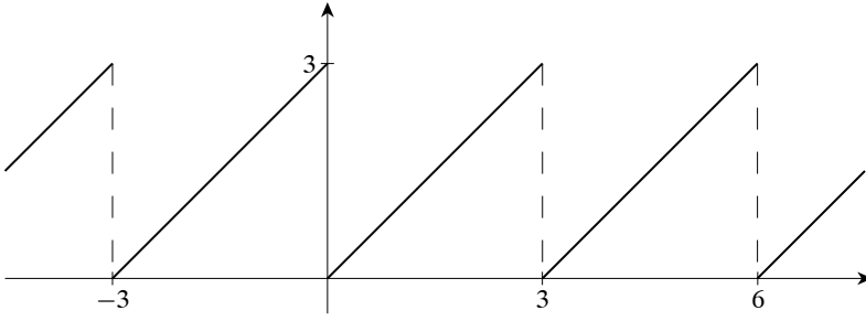
Figure 36.2: The graph of \text{saw}_3 .
