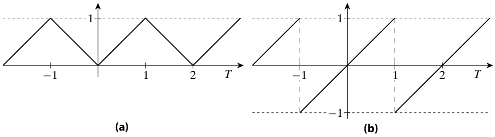
Figure 36.4: Two and one half periods of (a) \text{evensaw}(t) , the even sawtooth function for exercise 36.12 c, and (b) \text{oddsaw}(t) , the odd sawtooth function for exercise 36.12 d.
