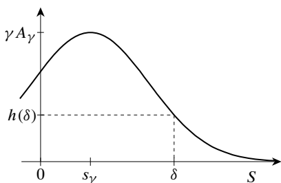
Figure 26.2: The shifted Gaussian h(s) when s_{\gamma} < \delta .
