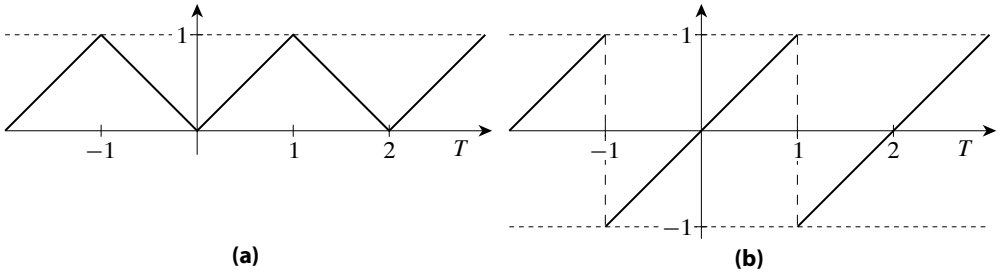
Figure 27.4: Two and a half periods of (a) \text{evensaw}(t) , the even sawtooth function, and (b) \text{oddsaw}(t) , the odd sawtooth function for exercises 27.18 c and 27.18 d.
