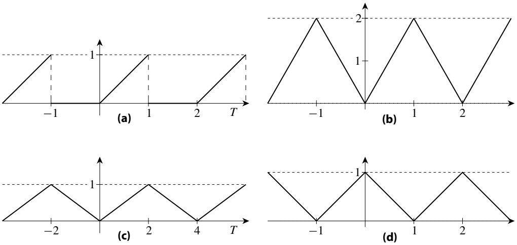
Figure 9.5: Two and one half periods of (a) \Phi(t) , the broken sawtooth function for exercise 9.7 d, (b) \Psi_1(t) , the scaled even sawtooth function, for exercise 9.7 e, (c) \Psi_2(t) , the scaled even sawtooth function for exercise 9.7 f, and (d) \Psi_3(t) , the shifted even sawtooth function for exercise 9.7 g.
