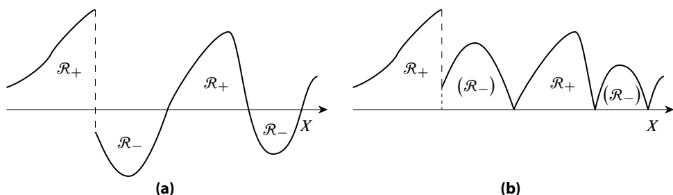
Figure 18.1: (a) The graph of some real-valued function f and (b) the graph of its absolute value.
