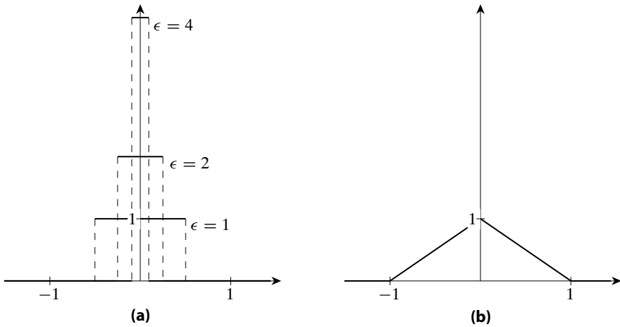
Figure 26.1: Some functions in two identity sequences — (a) \frac{1}{2\epsilon} pulse _{\epsilon} for various values of \epsilon , and (b) the basic triangle function, tri, from example 26.3.
