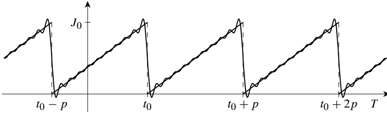
Figure 13.4: Graphs of a shifted and scaled saw function and a partial sum approximation to its Fourier series.
