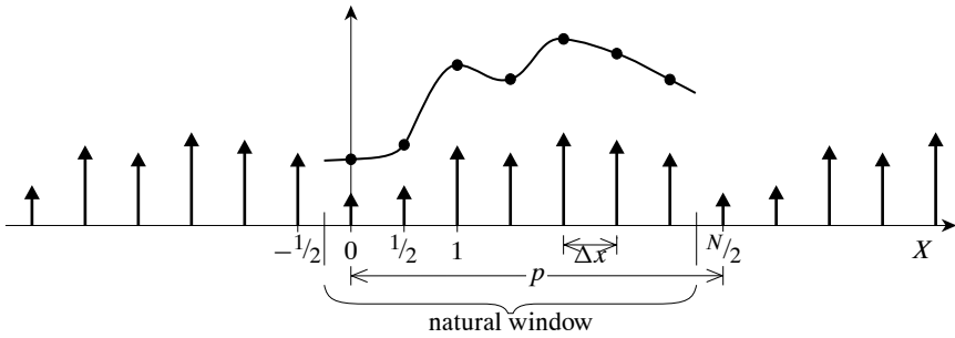
Figure 39.2: The discrete approximation for the function and sampling from figure 39.1 assuming that \Delta x = 1/2 . The sampling and the graph of the function over the natural window have also been sketched.
