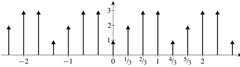
Figure 38.2: The periodic, regular array for example 38.1.
