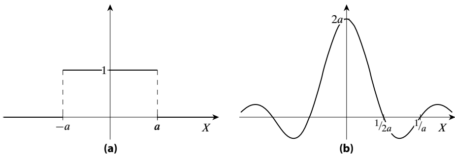
Figure 19.1: The graphs of (a) pulse a (x) and (b) its Fourier integral transform, 2a sinc(2πax). (These graphs correspond to a ≈ 1.)
