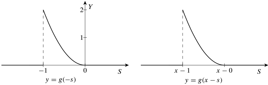
Figure 24.2: Steps 2 and 3 in computing f * g(x) — graphing g(-s) and g(x-s) .
