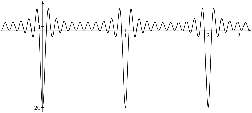
Figure 15.1: Graph of S_{10} from example 15.1 (with vertical axis compressed).
