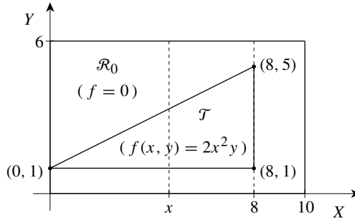
Figure 7.1: Figure for example 7.2.
