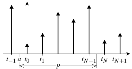
Figure 38.3: Choosing a ( t_k = k\Delta t ).
