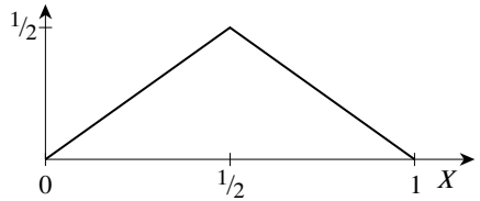
Figure 16.1: The initial shape of the string in example 16.2.
