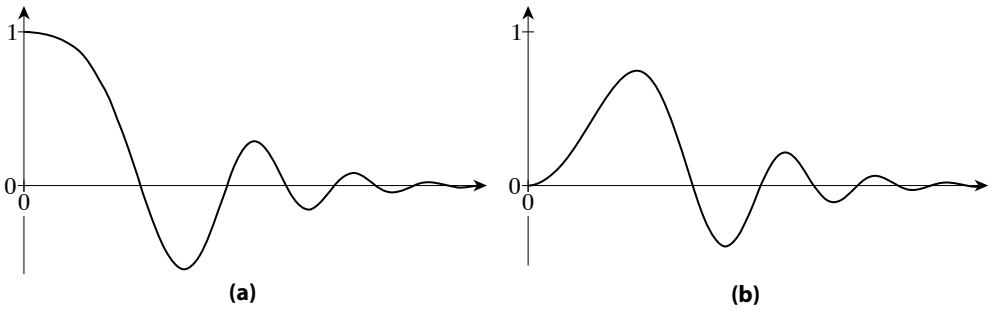
Figure 23.2: Graph of (a) the real part and (b) the imaginary part of e^{-(\gamma+i\kappa)x^2} with \gamma > 0 and \kappa > 0 .
