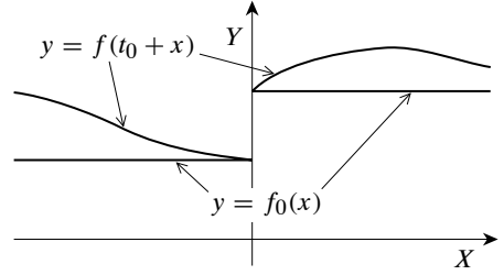
Figure 14.1: f and f_0 .
